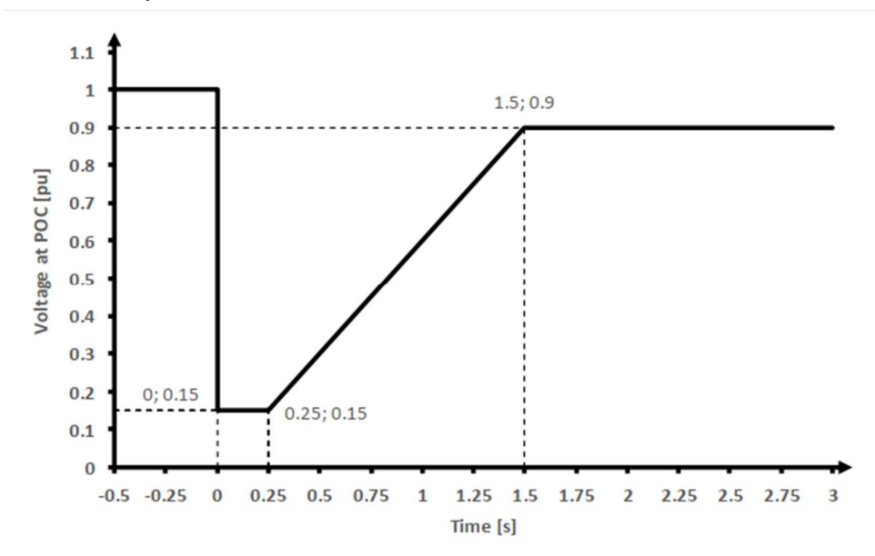
Figure 5.2—Tolerance to voltage dips for a power park module.
