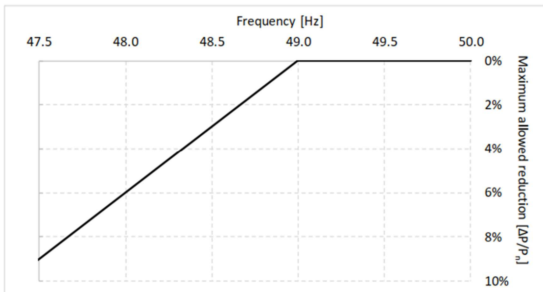
Maximum allowable power reduction in case of under-frequency
