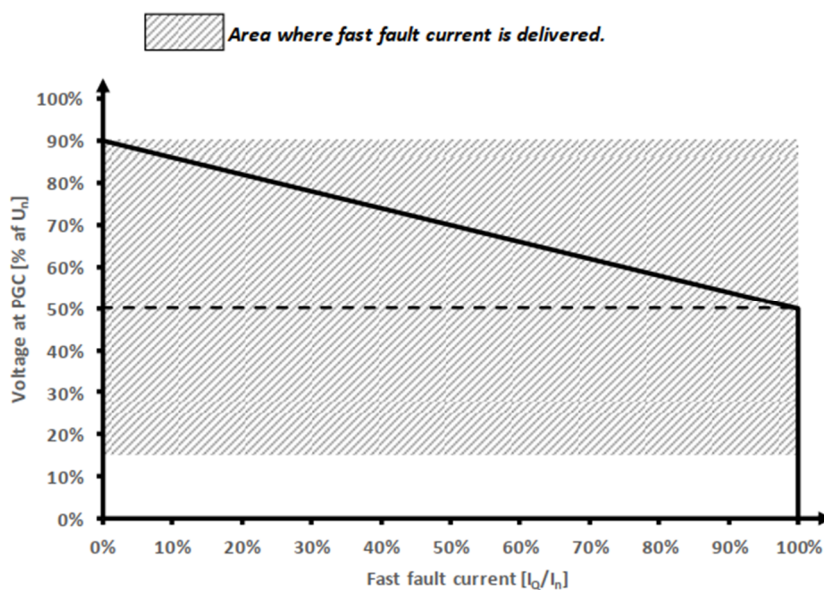
Figure 12 —Supply of fast fault current from a power park module
