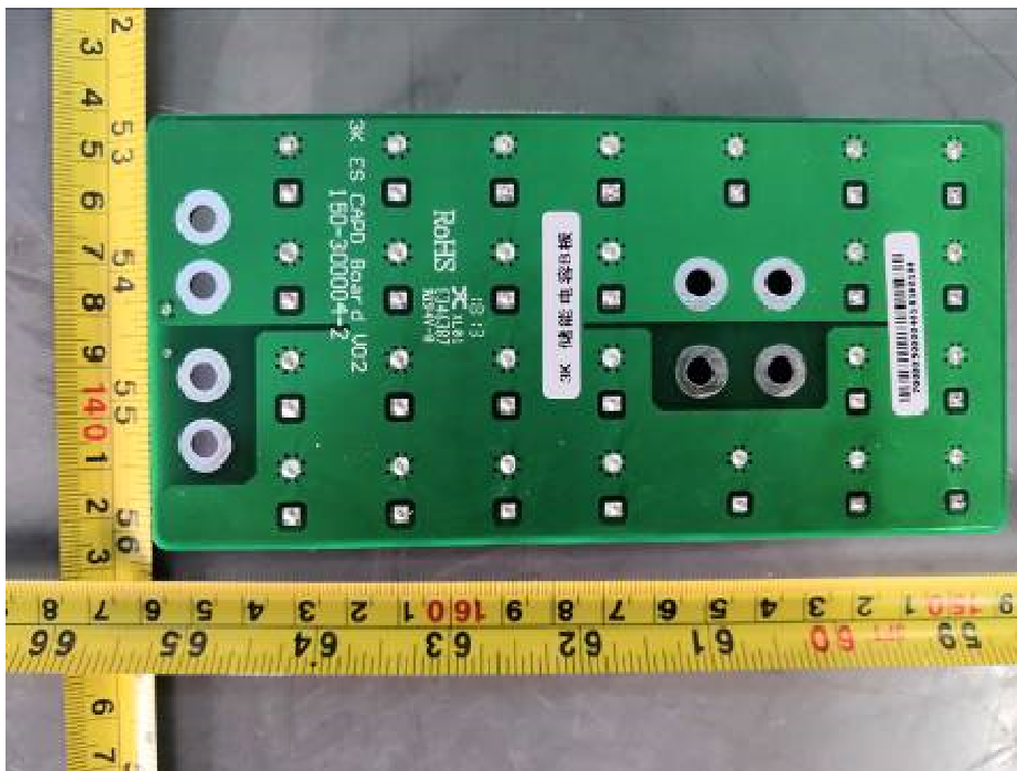
Capcintance B board solder side view
